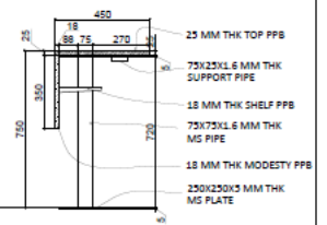
SECTION
