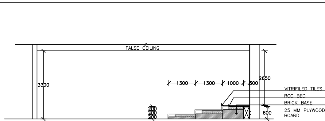
SECTION - A
